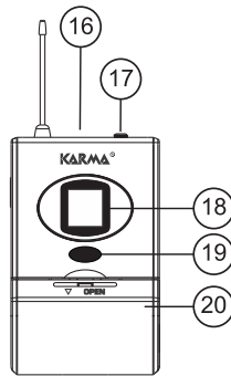
Bodypack microphone
