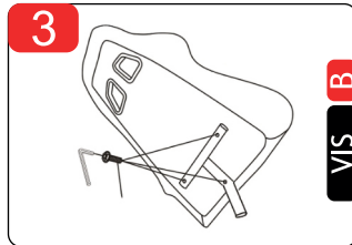
3 Screw the T-bar to the backrest (groove towards the outside)
