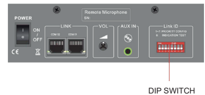
DIP SWITCH
